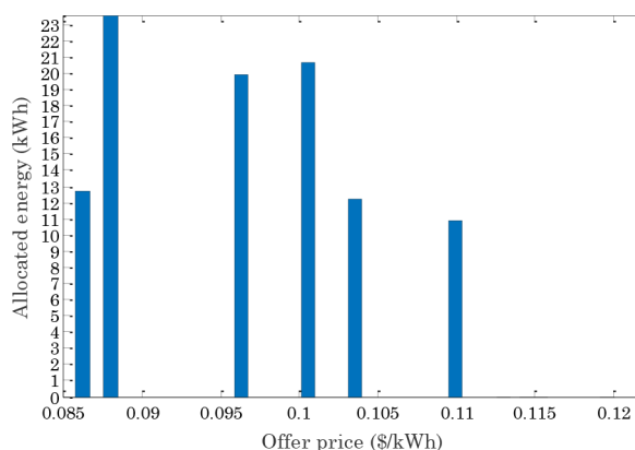
Fig. 5. Blockchain-inspired auction mechanism
